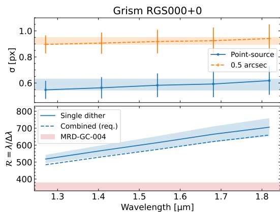
Fig. 12: Top : distribution (median \pm sMAD) of intrinsic spectral resolution \sigma (in blue) and effective 0''.5 -source \sigma_e (in orange) for RGS000+0 (pointing ID 266626). Bottom : corresponding resolving power \mathcal{R} , for a single-dither spectrum (continuous line) and a 4-dither combined spectrum (dashed line), assuming an as-required wavelength accuracy (38% of a resolution element, see text); the red zone corresponds to the requirement from top-level mission document.
